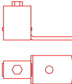
Connector Lug Assembly 400 amp PN 250005
