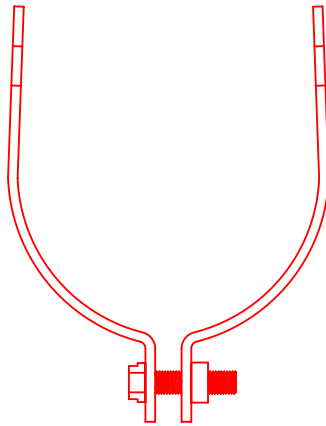
3" 2 Piece Metal Clamp (2 per Cell) PN 310010
