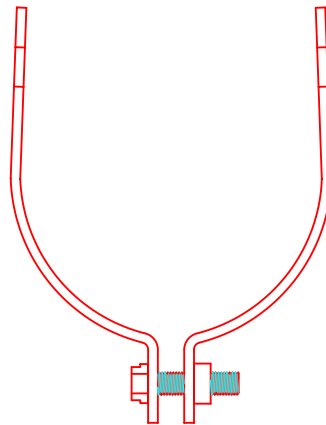
2" 2 Piece Metal Clamp (2 per Cell) PN 310012
