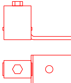
Connector Lug Assembly 225 amp PN 250001
