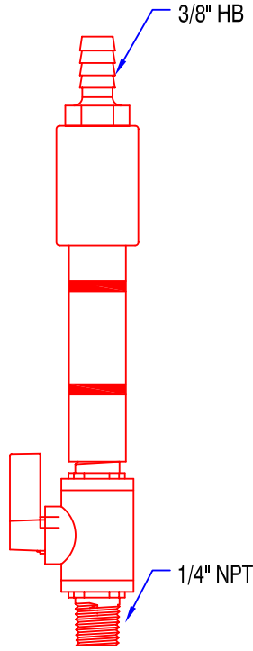
PVC Shut Off Valve/Flowmeter PN 225010
