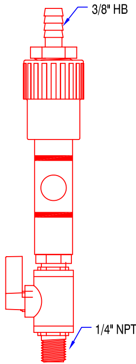
PVC Shut Off Valve/Flowmeter PN 225042
