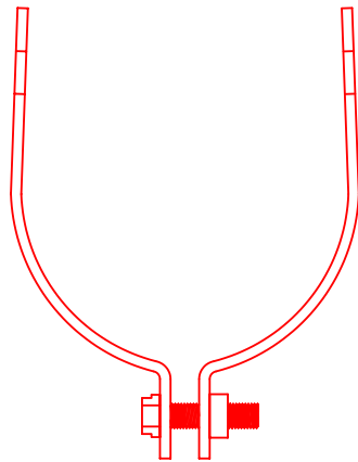
2" 2 Piece Metal Clamp (2 per Cell) PN 310012
